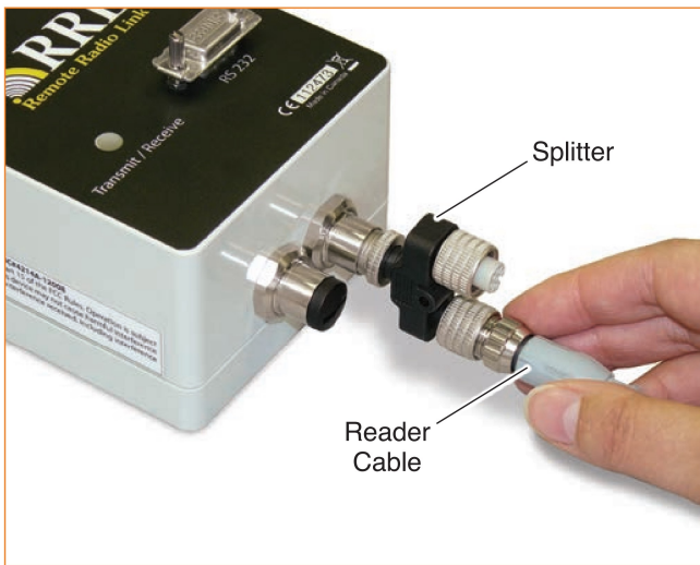
Position the Splitter as shown in the photo above to accommodate two Splitters on the RRL Station.
