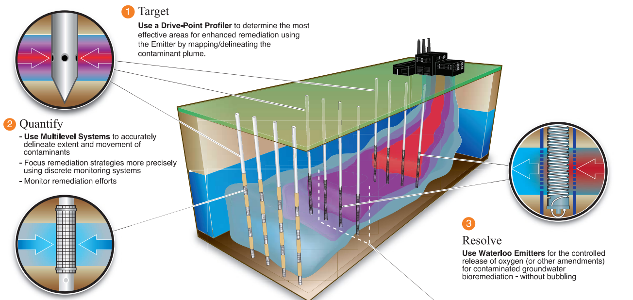
Multiple Well Installation with a Single Gas Supply
