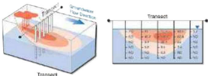
Multilevels Provide Three Dimensional Groundwater Data. Illustration courtesy of LFR Levine-Fricke and the American Petroleum Institute
